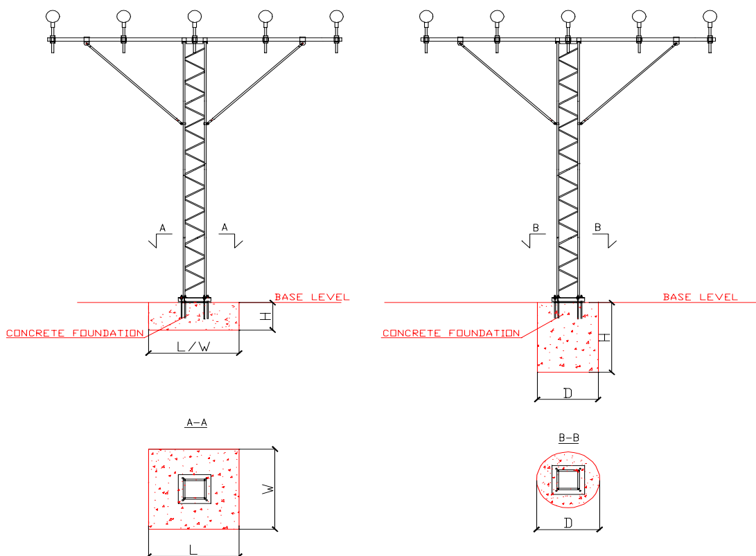
Illustration 2: Slab foundation and drum foundation
