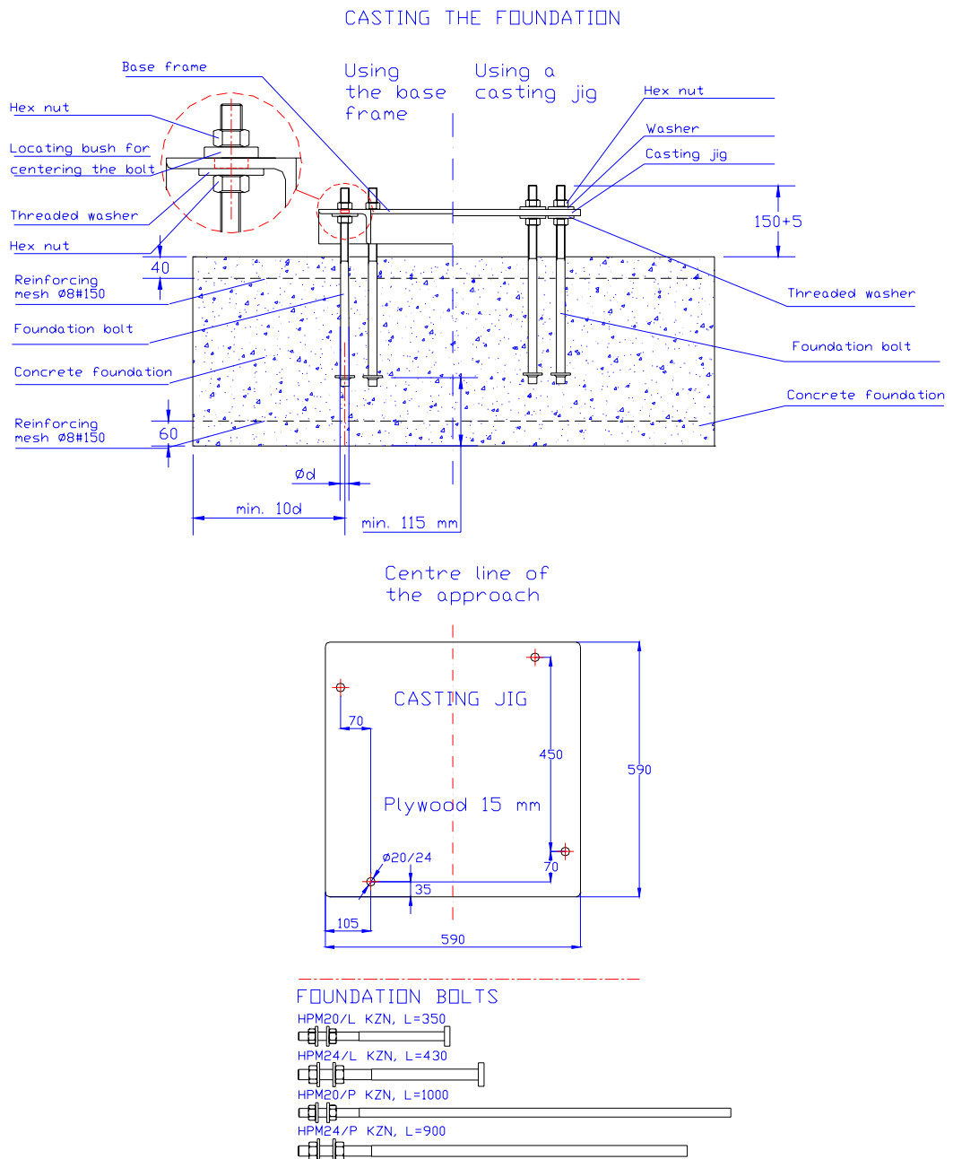
Illustration 3: Principal draft of foundation, casting jig and foundation bolts of the mast.
